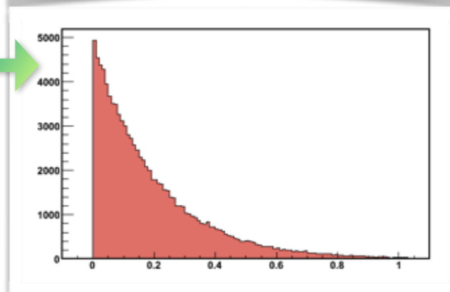
Exponential
