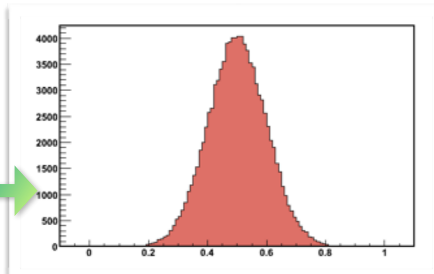
Gaussian
